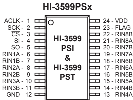
24 - Pin Plastic Small Outline Package (SOIC)
