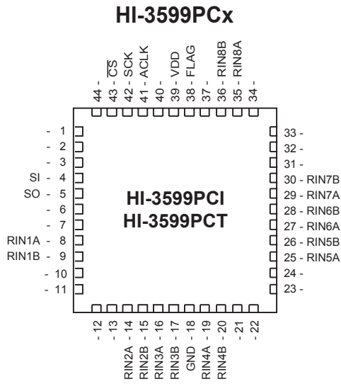
44-Pin Plastic 7mm x 7mm Chip-Scale Package (QFN)
