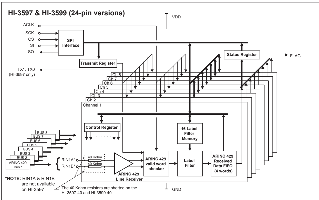
Figure 1. Block Diagrams
