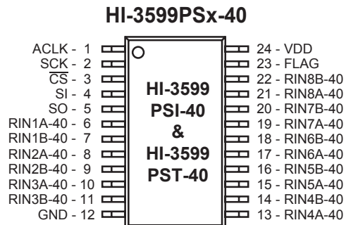
24 - Pin Plastic Small Outline Package (SOIC)
