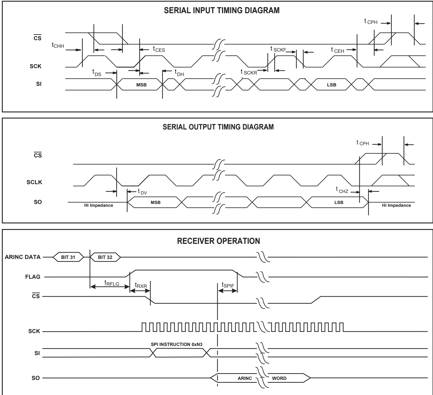
Figure 5. Timing Diagrams
